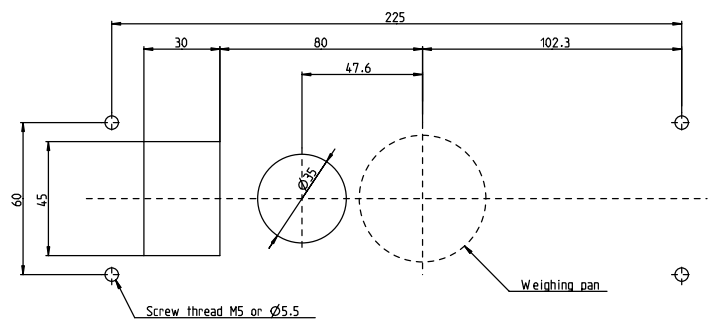
Hole pattern (mm)
