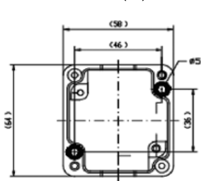
Dimensions Terminal Box (mm)
