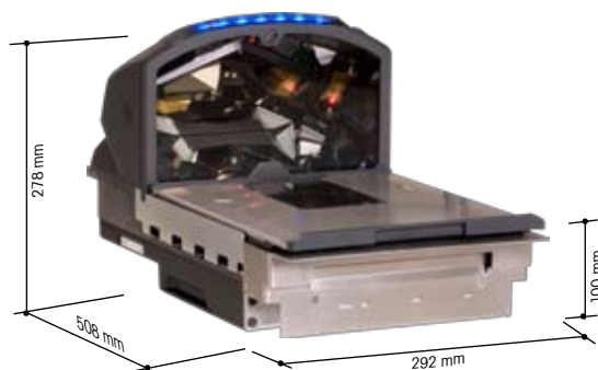
Stratos H Dimensions - 2300 Series
